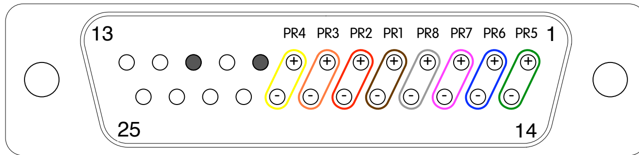
Rear View (wiring side)
